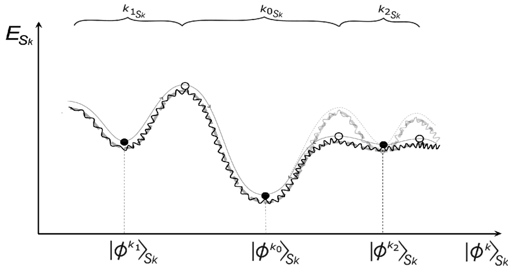
Figure 2. Schematic presentation of the adaptation of memory attractors in the energy-state hypersurface of the quantum-holographic memory / propagator of various hierarchical levels of biological macroscopic open quantum system(s) S_k [13,14,49] (local cell's biomolecular protein / target, local acupuncture system / consciousness, or nonlocal out-of-body consciousness / collective consciousness). This implies necessity of quantum-informational successive bioresonant balancing of all unwilling side memory attractors (like \phi^{k_2} in Fig. 2), which would otherwise cause development of psychosomatic diseases on the individual level, and interpersonal fights in this and further generations on the collective level. 18,19
