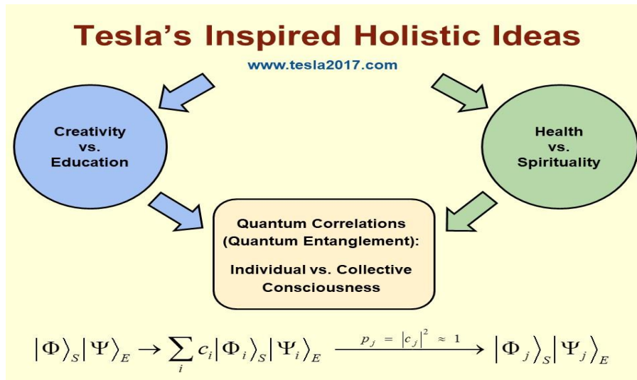
Figure 1. (a) Symbolic representation of mentally controlled-directed increasing of macro-quantum correlations of individual and collective consciousness in transpersonally entangling creative phases (left-hand side of the image and formula above, with previous mental increase of the focused weight contribution c_j and subsequent (practically non-stochastic) classically-reduced selection of this dominant weight contribution c_j ) [14,15]; and (b) Symbolic representation of mentally controlled-systemic decreasing of macro-quantum correlations of individual and collective consciousness in transpersonally disentangling spiritual phases (right-hand side of the image and formula above, with previously systemic mental decreasing of almost all weight contributions c_i and subsequent (practically non-stochastic) classically-reduced selection of the remaining dominant weight contribution c_j (related to mentally-embedded address on the founder of the corresponding mystical tradition) [14,15]. 17
